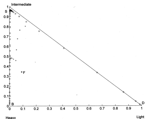
Fig. 3. Liquid composition profile in a thermally coupled gas concentration unit.
