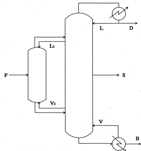
Fig. 1. Schematic of fully thermally coupled distillation system (F: feed; D: benzene; S: toluene; B: high b.p. product)
