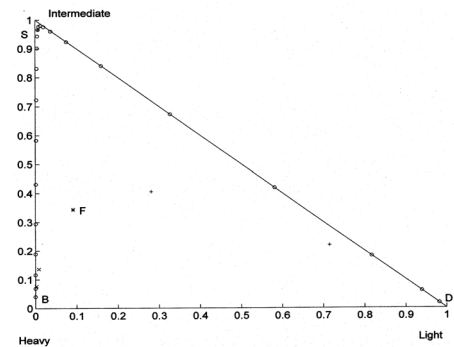
Fig. 2. Liquid composition profile in minimum trays.
