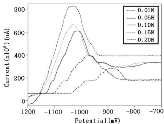
Fig. 3. Cyclic voltammogram of LB film of LLPC monolayer onto ITO glass at a various concentration of KClO_4 solution. The scan rate was 100mV/s.
