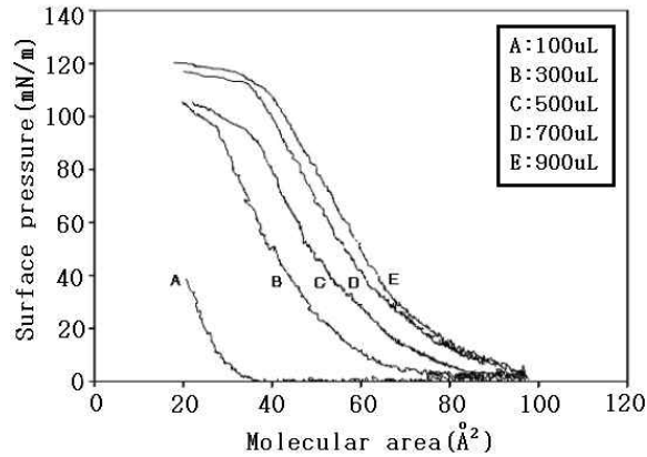
Fig. 2. \Pi -A Isotherm curves for LLPC.
